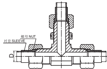
JIC 外螺纹 74° 外锥 JIC MALE 74° CONE
